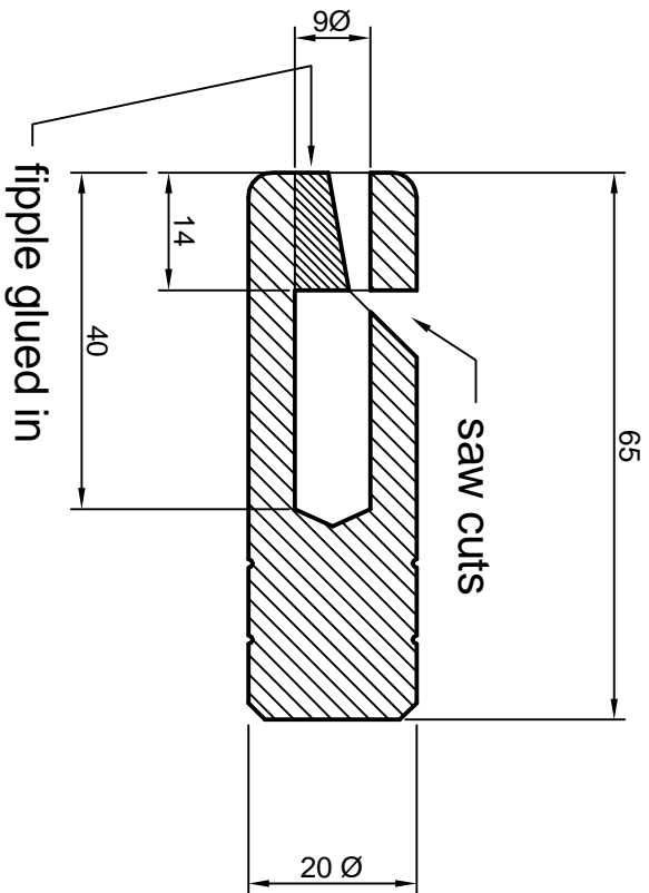
Section
